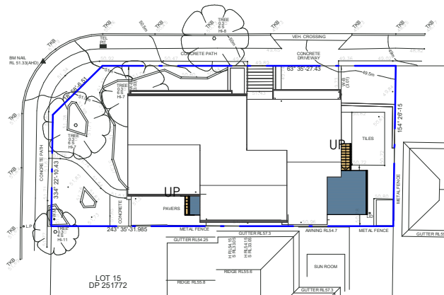
EXISTING SITE PLAN
